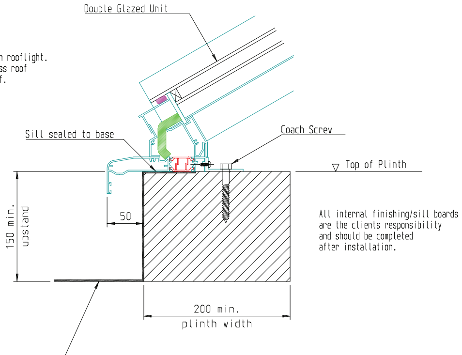
Roof Plinth detail A-A Scale 1:5
